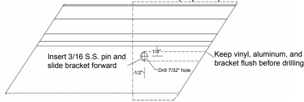
Contour Stair Bracket (Top Rail)
